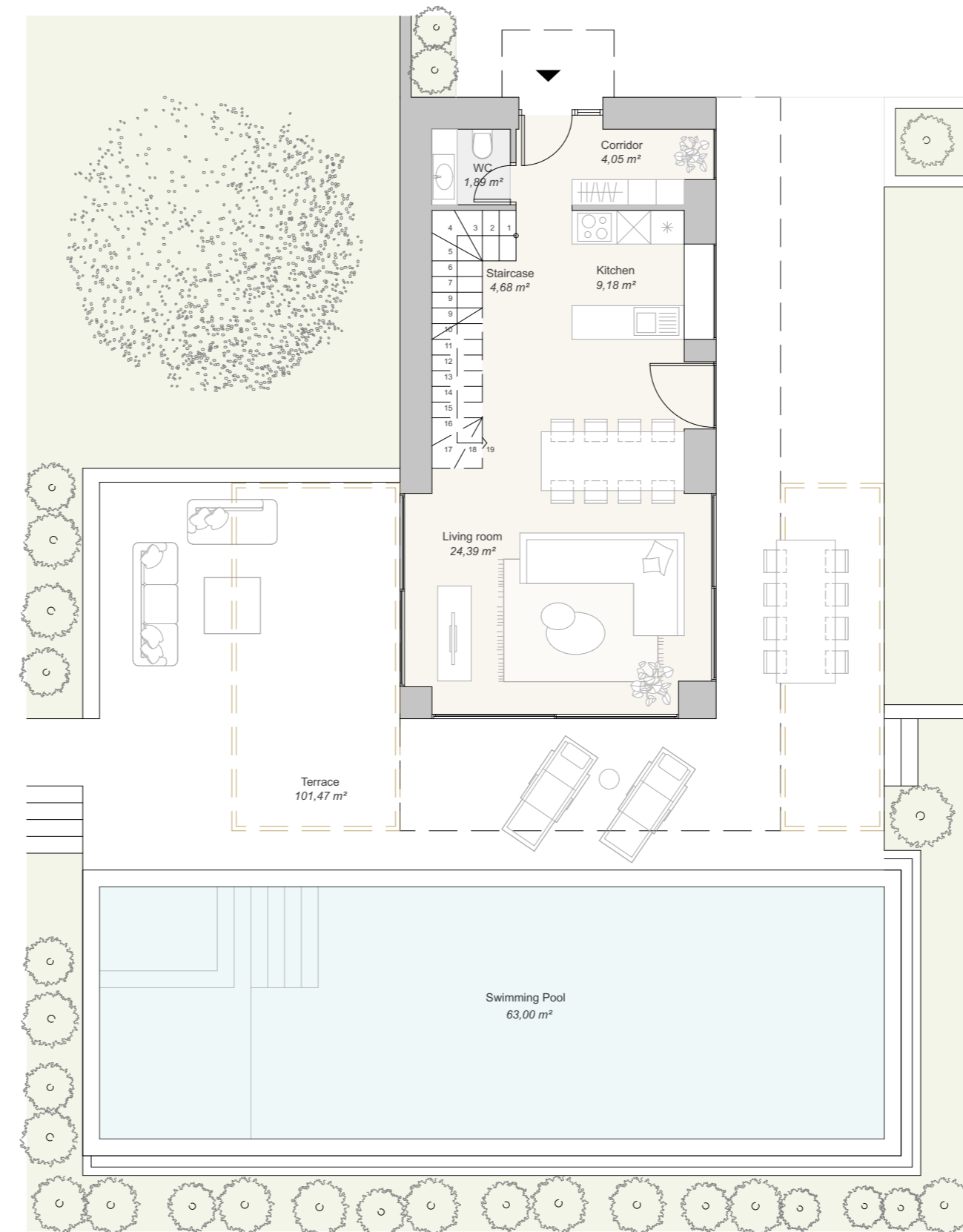
Groundfloor
