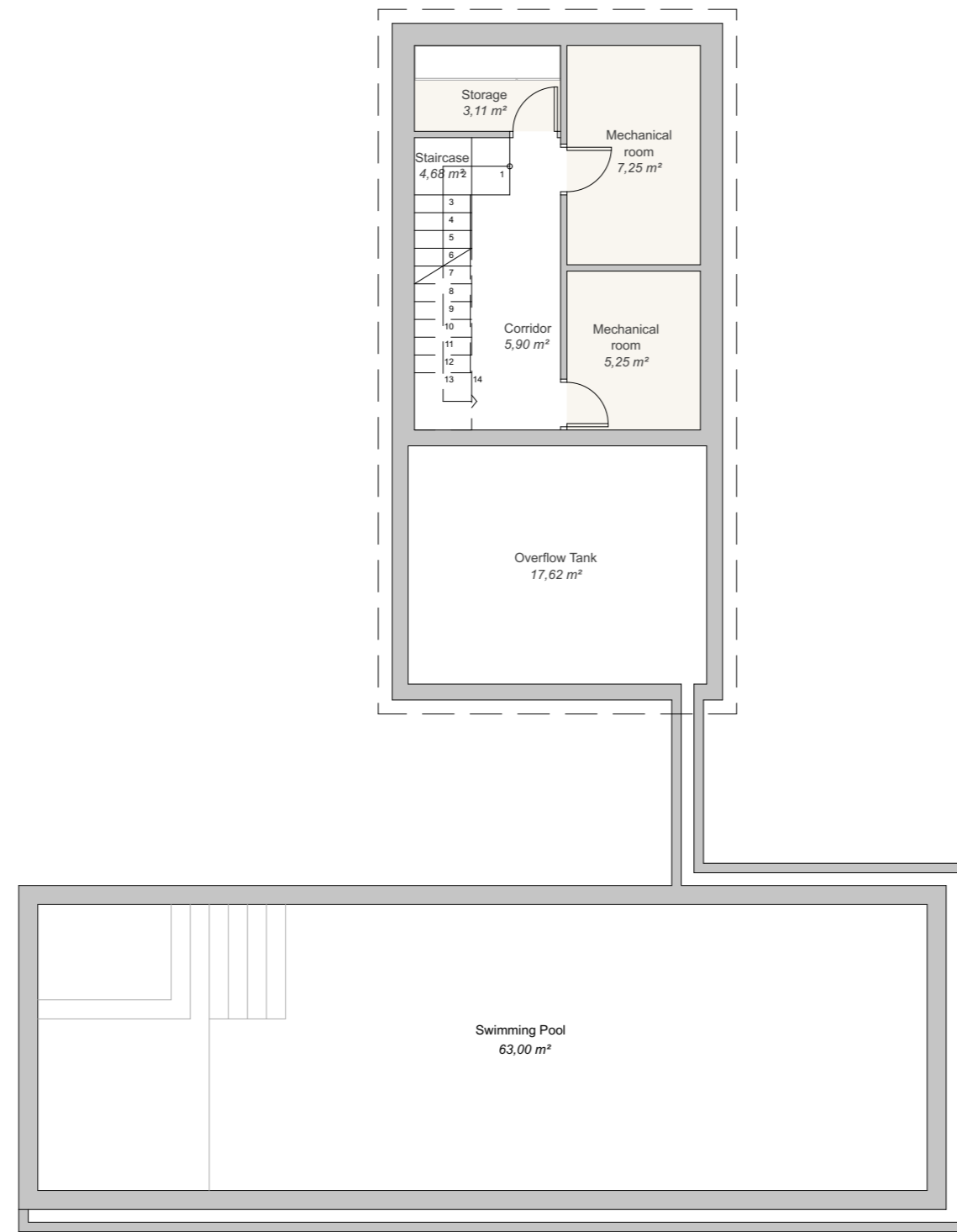
Basement
